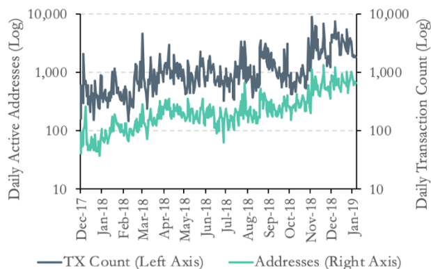
FIGURE 7A Dai Active Addresses & Transaction Counts
