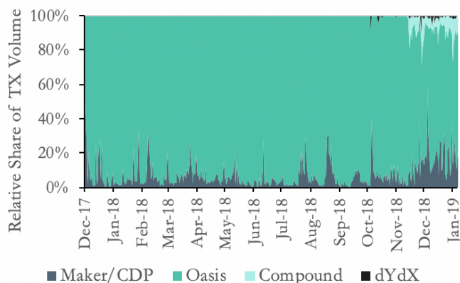
FIGURE 8B Relative Share of On-Chain TX Volume
