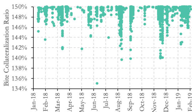
FIGURE 5A CDPs by Bite Collateralization Ratio
